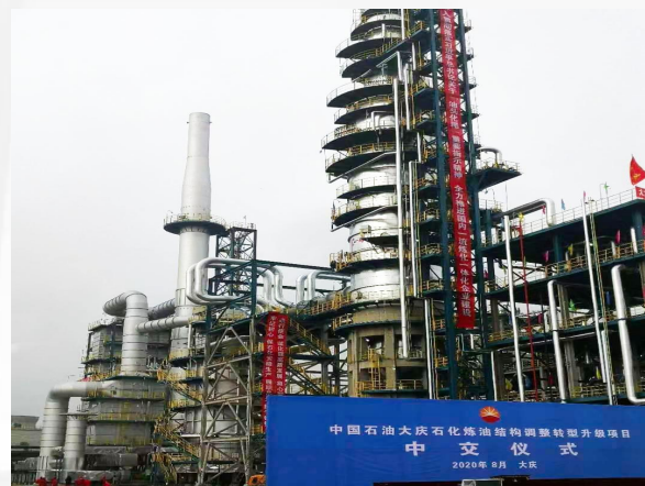
常减压加热炉 Atmospheric and vacuum heater
