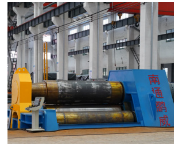
Intelligent CNC four-roll plate rolling machine
