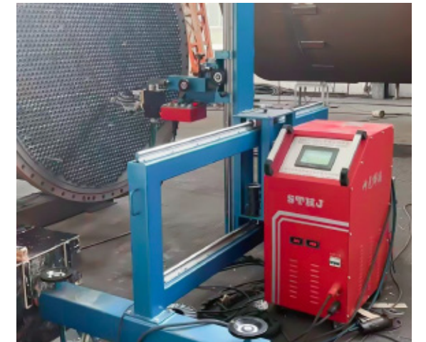
Tube sheet automatic welding machine
